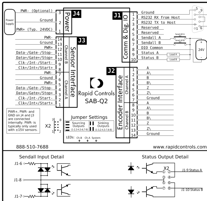
Figure 1: SAB-Q2 Connector and Jumper Placement
